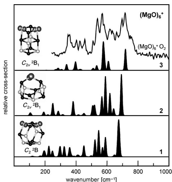
Figure 3. The IR-MPD spectrum of the (\text{MgO})_6^+ cluster ion and the calculated linear IR absorption spectra for its three most stable structural isomers. The relative energies of the isomers are given in Table 1.
