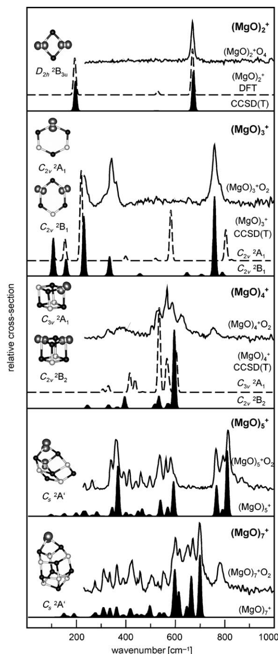
Figure 2. Comparison of the experimental IR-MPD and calculated linear IR absorption spectra for the most stable (\text{MgO})_n^+ gas-phase clusters with n=2 –5 and 7 along with their geometrical structures. The calculated CCSD(T) and the DFT (B3LYP) spectra are shown for n=2 –4 and n=2, 5 , and 7, respectively. The calculated spectra are convoluted with Gaussian functions. (Mg: black spheres, O: white spheres, isosurface of spin density: gray).
