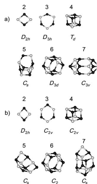
Figure 1. The most stable structures of a) neutral (\text{MgO})_n and b) cationic (\text{MgO})_n^+ clusters with n = 2–7 (black: Mg, white: O).
